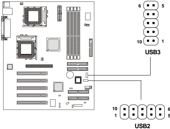
USB2 Pin Definition
