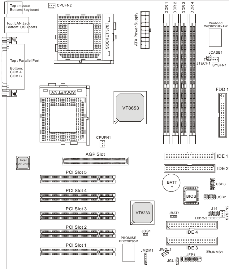
Pro266TD Master-LR (MS-9105) ATX Mainboard
