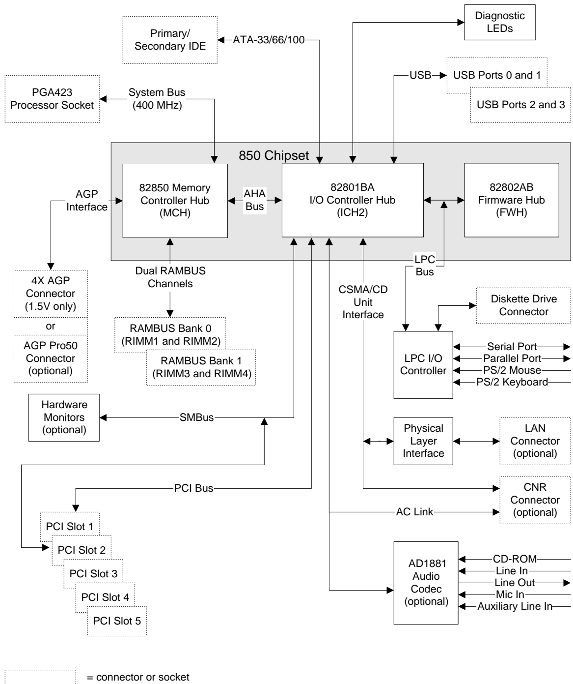
Figure 2. Block Diagram
